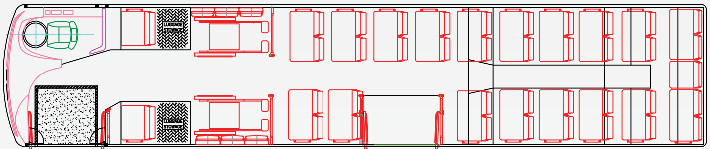
SEAT CONFIGURATION 45 SEATED PASSENGERS 2 WHEELCHAIR POSITIONS 2 DOORS
